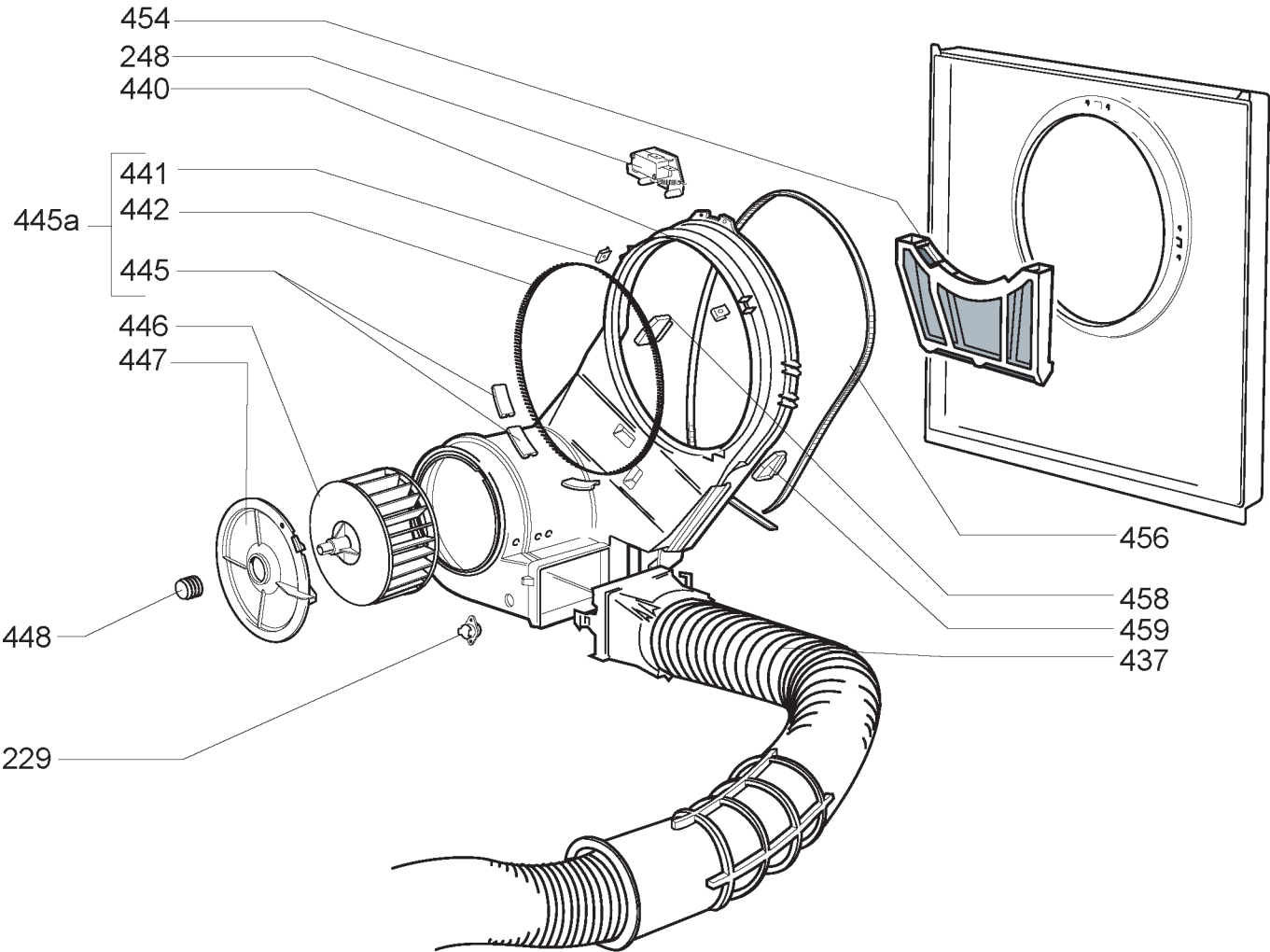
White Knight Electronic Sensing Air Vented Dryer - Exploded View 2
