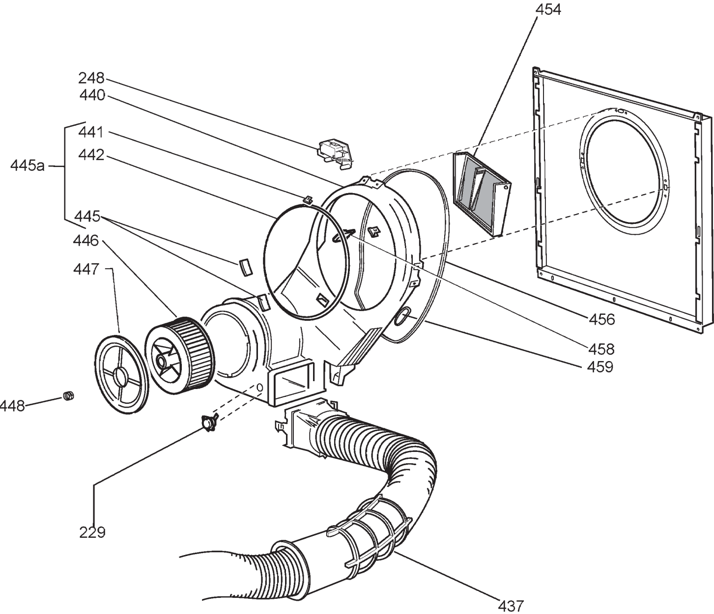
White Knight - Air Vented Tumble Dryer - Exploded View 3
