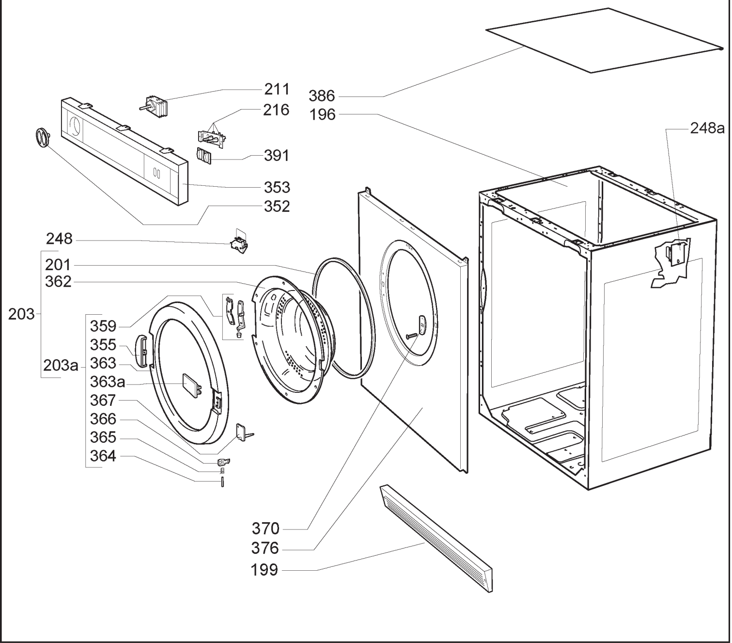
White Knight Exploded View 1
