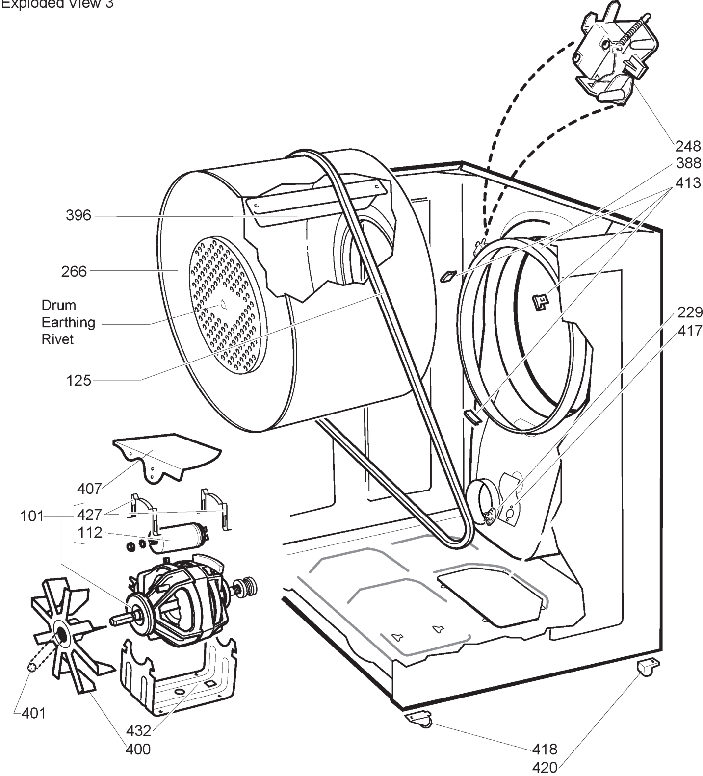
Exploded View 3
