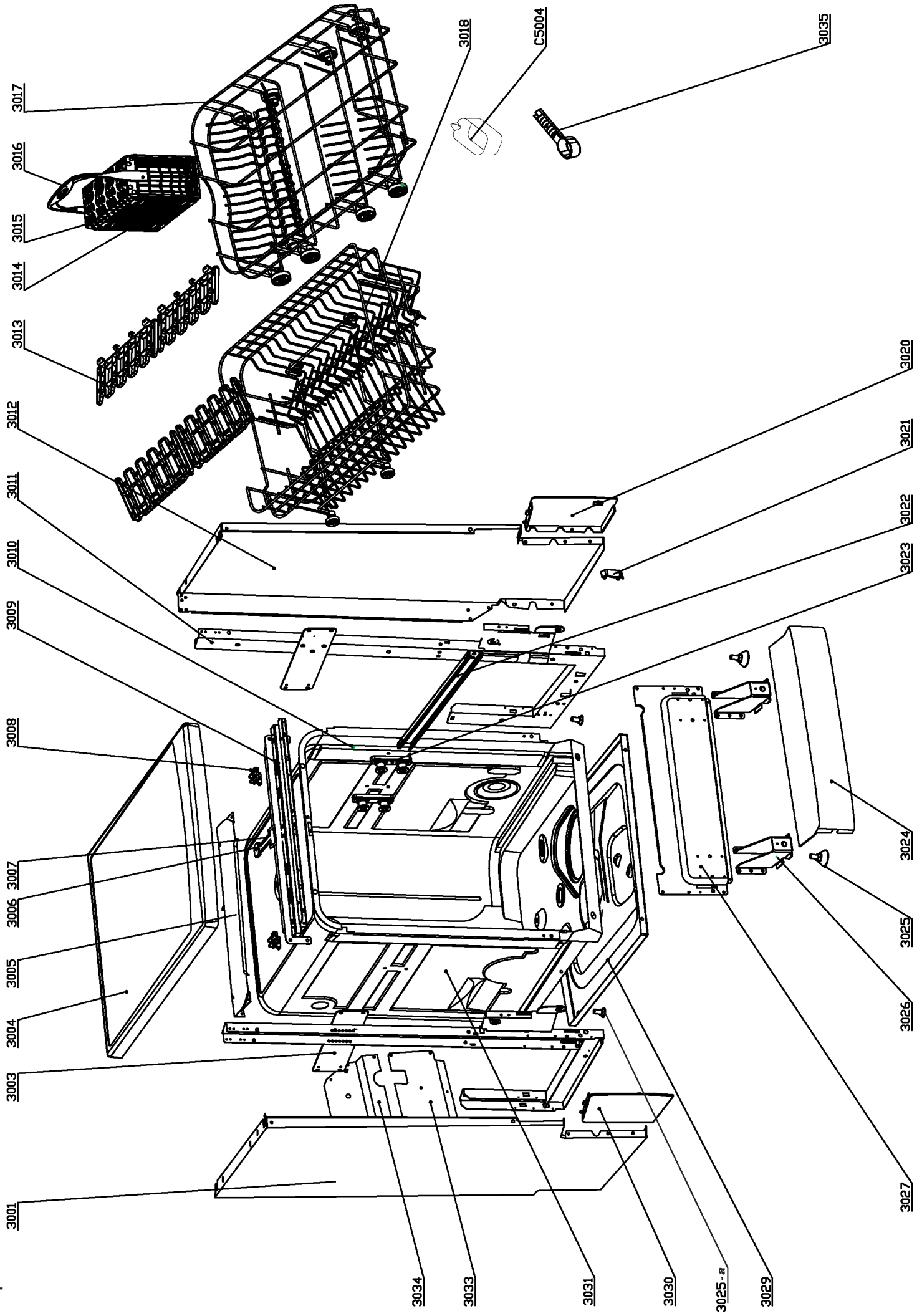
Exploded View 3
